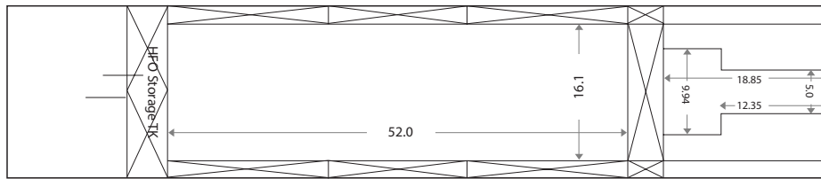
TANK TOP
